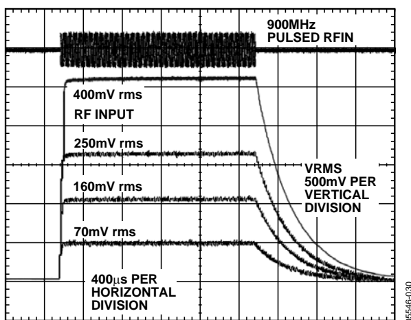
Figure 30. Output Response to Modulated Pulse Input for Various RF Input Levels, Supply 3 V, Modulation Frequency 900 MHz, 0.01 μF Filter Capacitor
