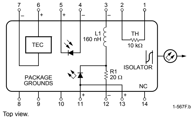
Figure 1. Circuit Schematic
