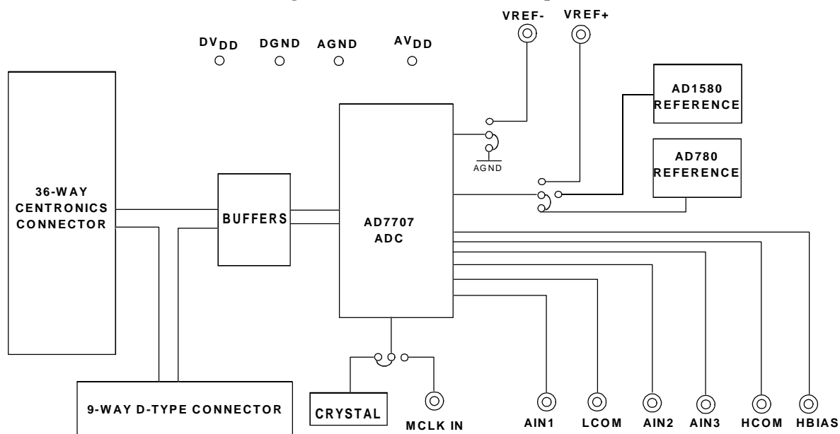
Figure 1: Evaluation Board Setup
