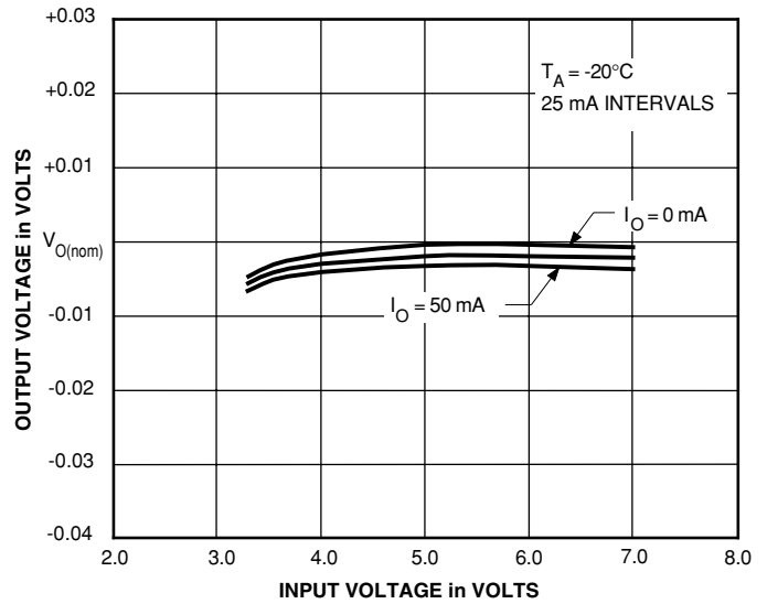
LINE REGULATION
