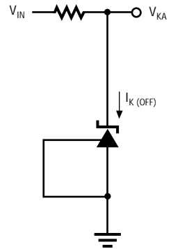
Figure 1c. Test Circuit 3
