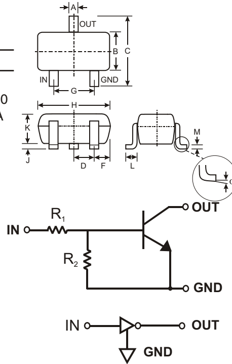
SCHMATIC DIAGRAM
