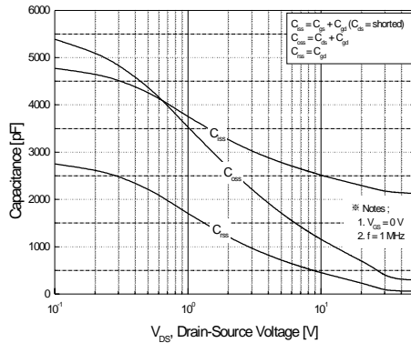
Figure 5. Capacitance Characteristics
