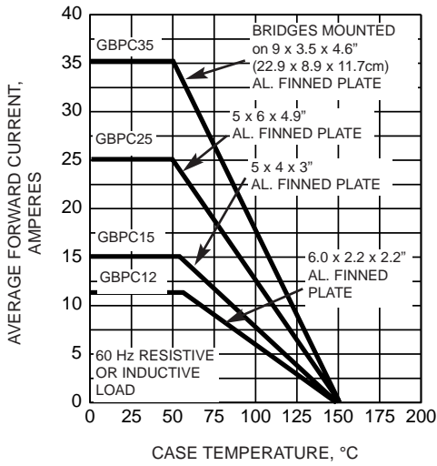
FIG. 1 - MAXIMUM OUTPUT RECTIFIED CURRENT
