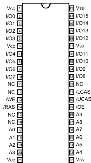
(Top View) 42 SOJ
