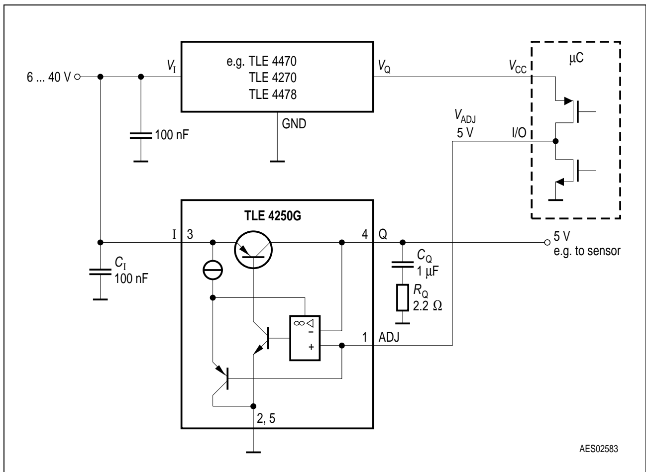
Figure 3 Application Circuit
