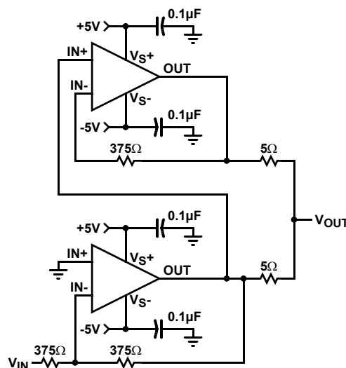
FIGURE 23. INVERTING 200mA OUTPUT CURRENT DISTRIBUTION AMPLIFIER
