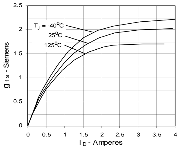
Fig. 8. Transconductance
