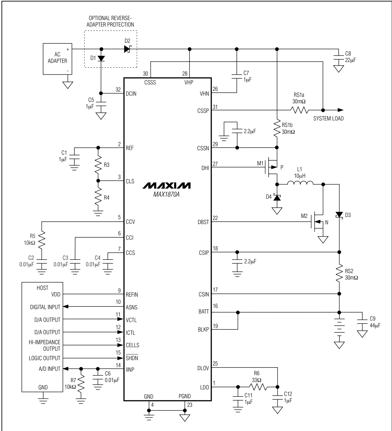
Figure 1. μC-Controlled Typical Application Circuit
