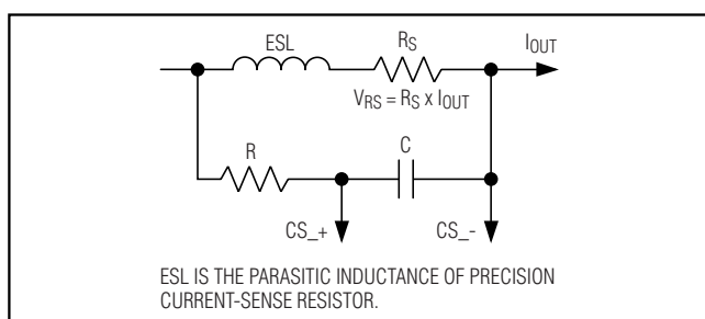
Figure 2. Current-Sense Resistor
