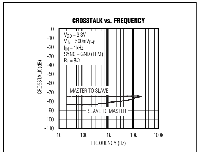
Figure 8. Master-Slave Crosstalk
