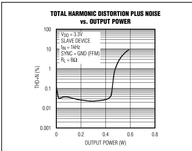
Figure 7. Master-Slave THD+N
