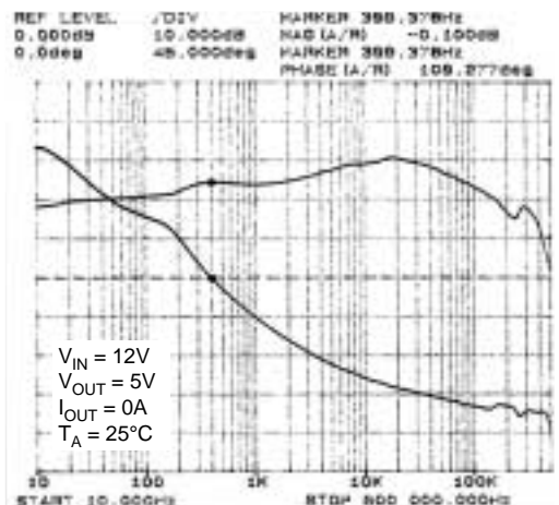
No-Load Stability Phase Margin = 109 ^{\circ}
