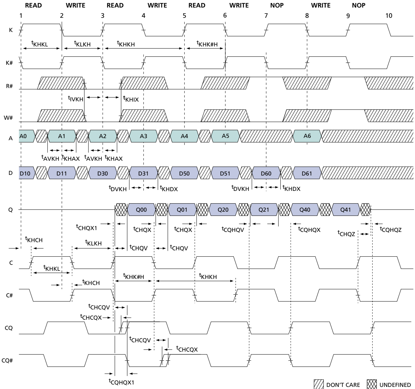
Figure 6: READ/WRITE Timing
