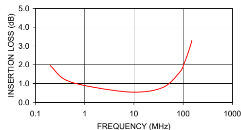
T14-1-KK81 INSERTION LOSS
