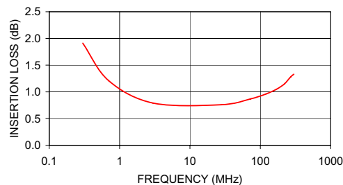
T5-1T-KK81 INSERTION LOSS
