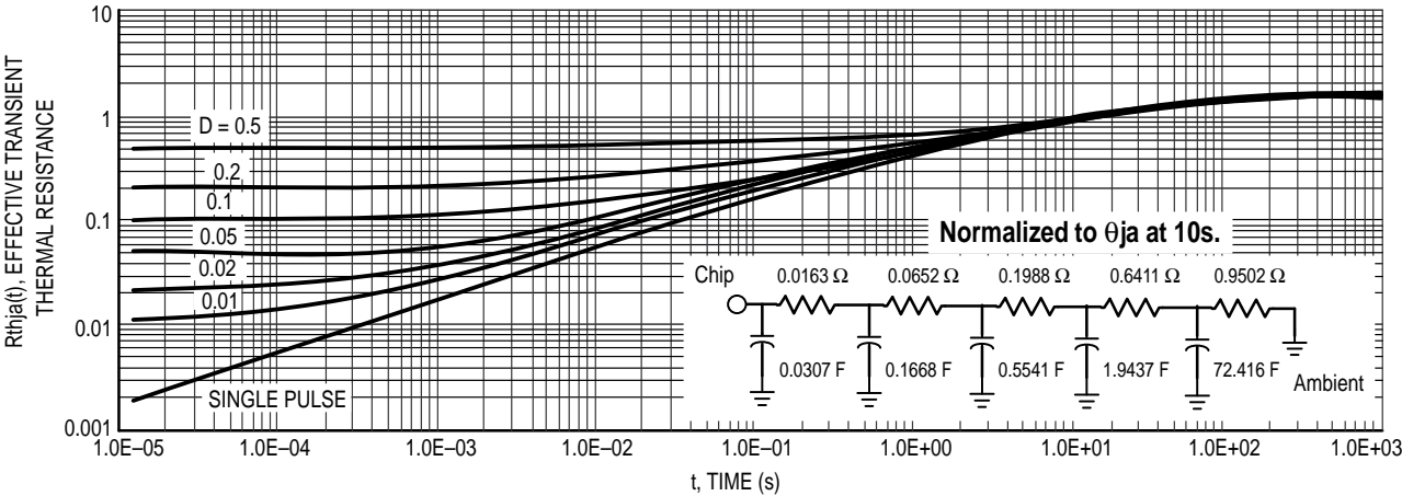
Figure 14. Thermal Response
