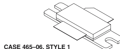
CASE 465-06, STYLE 1 NI-780 MRF5S19090L
