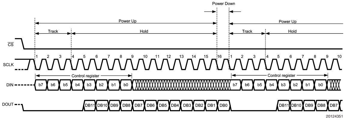
ADC124S021 Operational Timing Diagram
