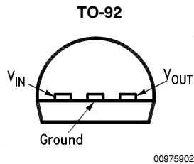
Bottom View Order Number LM2936Z-5.0 See NS Package Number Z03A
