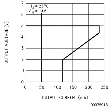
Current Limit
