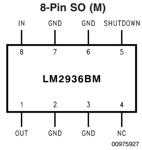
Top View Order Number LM2936BM-5.0 See NS Package Number M08A
