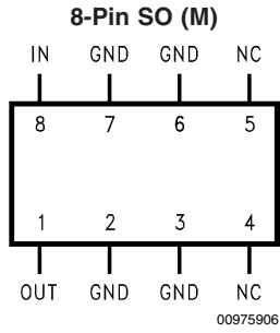
Top View Order Number LM2936M-5.0, LM2936HVMA-5.0 See NS Package Number M08A
