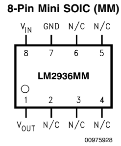
Top View Order Number LM2936MM-5.0 See NS Package Number MUA08A
