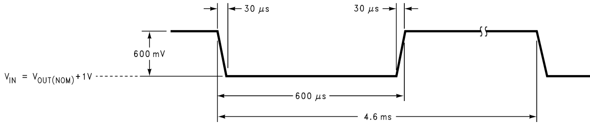
FIGURE 2. Figure 2. Line Transient Input Test Signal.
