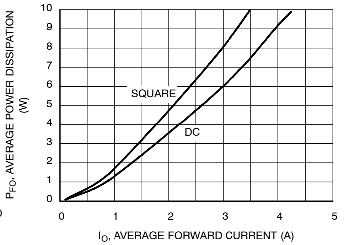
Figure 7. Forward Power Dissipation
