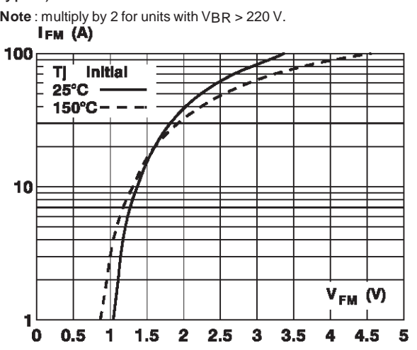
Fig. 5 : Peak forward voltage drop versus peak forward current (typical values for unidirectional types).
