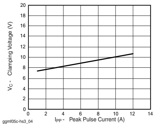
Fig. 4 Clamping Voltage vs. Peak Pulse Current
