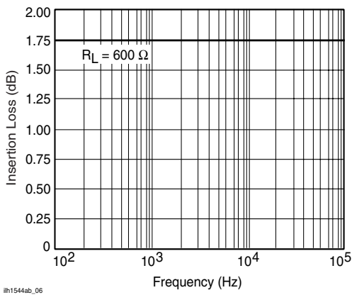
Figure 7. Insertion Loss vs. Frequency
